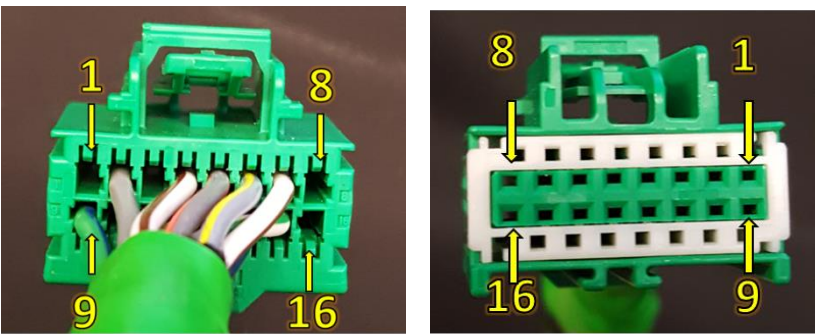
Green 16 Cavity VSIM Connector
