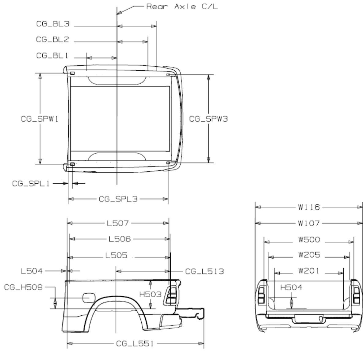
Ram 1500 (DT) 6' 4" Box Drawing
