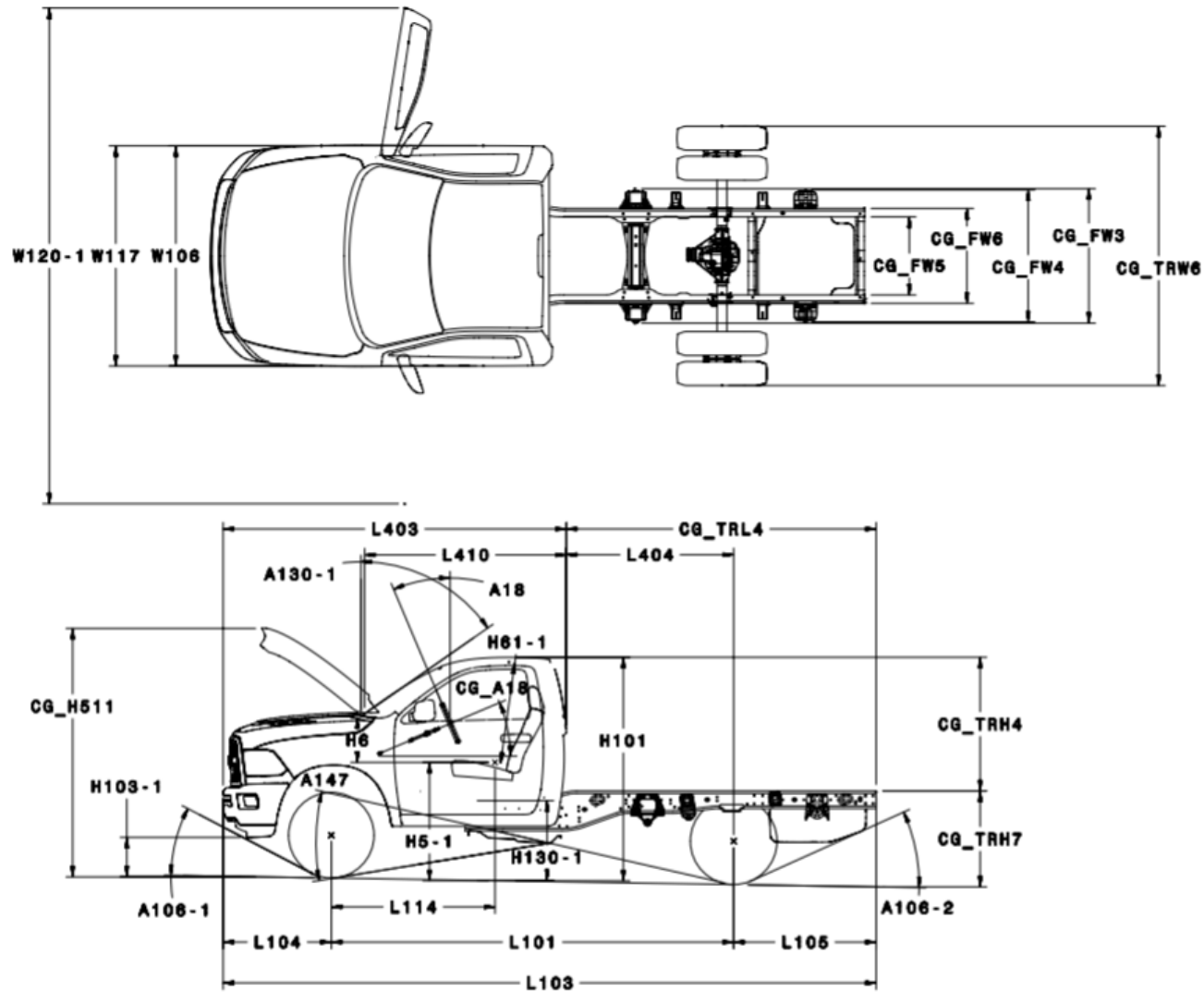
Views & Charts 2019 3500 Chassis Cab Reg Cab, 60CA, DRW
