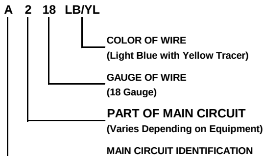
Figure 1 – Wire Color Code Identification
